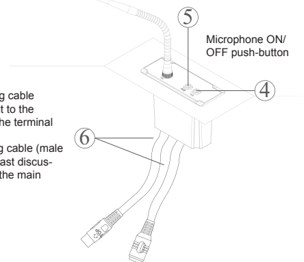
Embedding Installation Diagram
